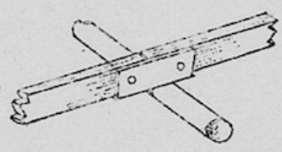
FIXING OF PURLINS
