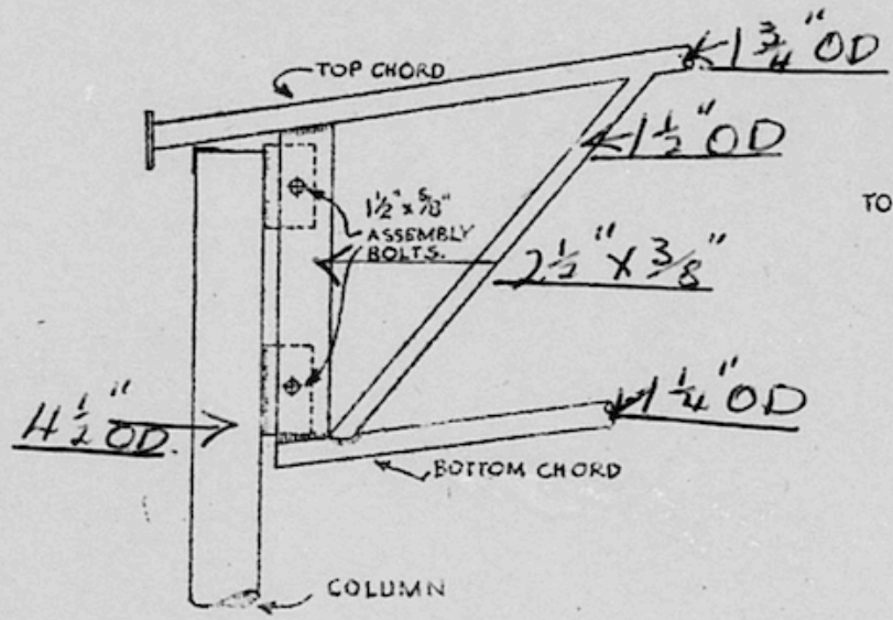
FIXING OF TRUSSES TO COLUMNS
