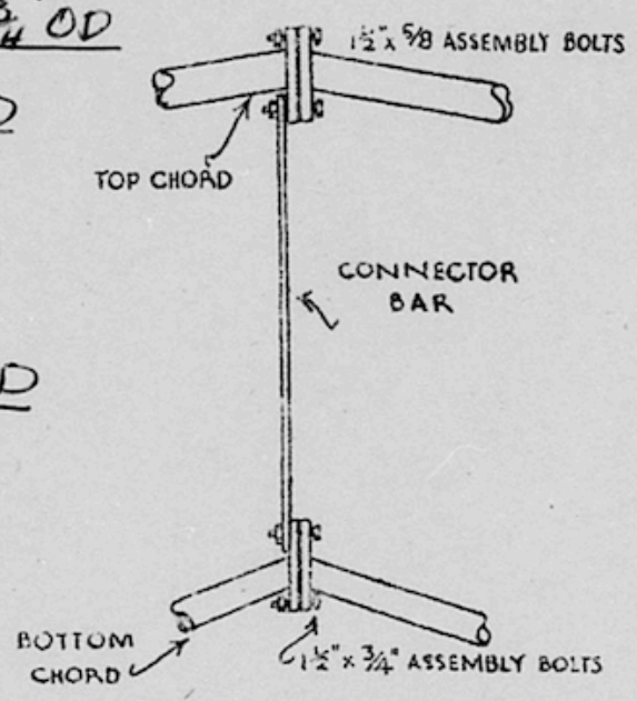
CENTRE ASSEMBLY OF HALF TRUSSES
