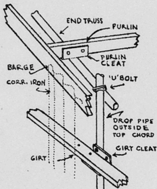
FIXING DROP PIPES & END TIMBERS
