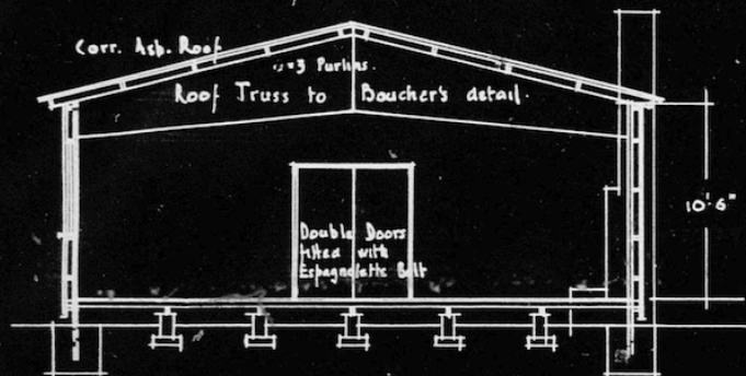
CROSS SECTION OF HALL
